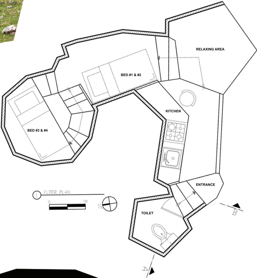
Floor Plan Area : 20 m 2
